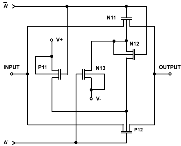
SWITCH CELL
